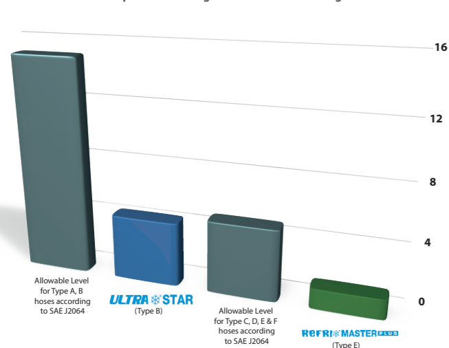
Comparison of Refrigerant Permeation Through Hoses
