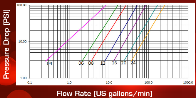
Pressure Drop
