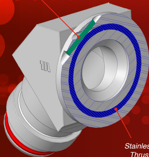
Stainless Steel Seloc Retaining Pin
