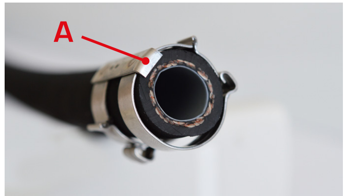
4 Place the double clamp on the hose so that the tooth on the bar (A) comes into contact with the end of the hose that has been cut
