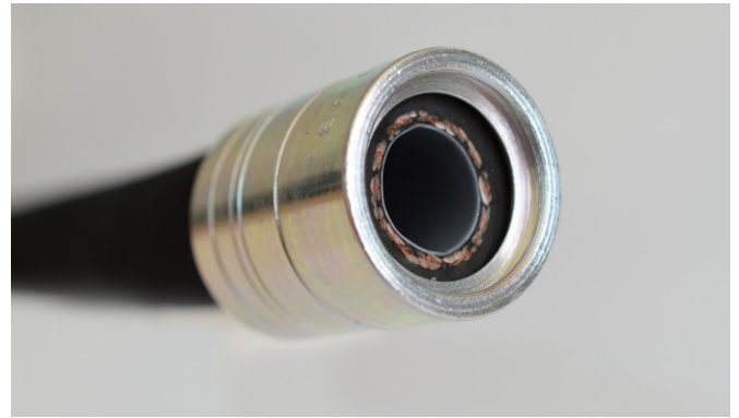
4 Place the ferrule on the hose so that the internal stop comes into contact with the end of the hose that has been cut
