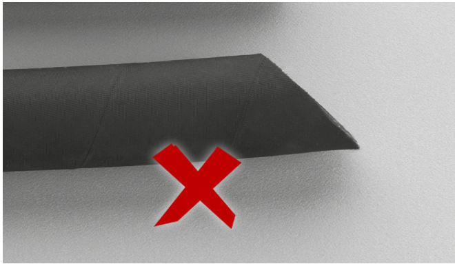
3 The end of the hose should be cut squarely to \pm 2^\circ
